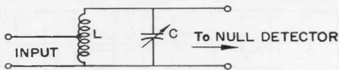
Figure 5. Simple tuned-circuit filter.
