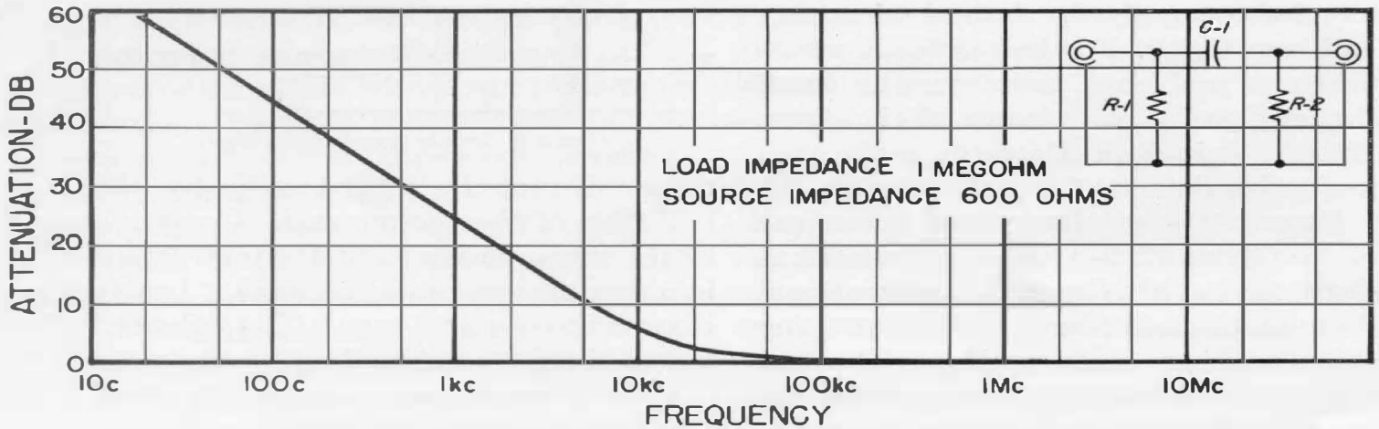
Figure 1. Attenuation characteristics of the Type 1212-P1 High-Pass Filter. The circuit diagram is shown at the upper right.
