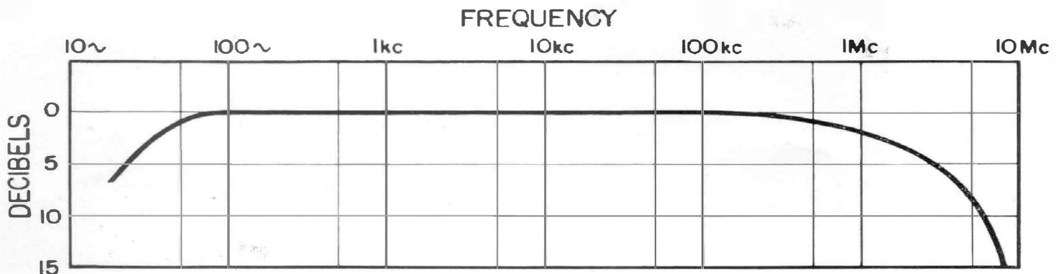
Figure 2. Frequency response characteristic of the Unit Null Detector.
