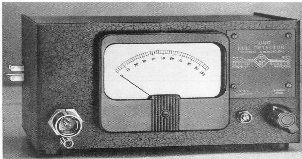
Figure 1. Panel view of the Unit Null Detector. The plug at the left connects to the Type 1203-A or Type 1204-B Unit Power Supply. At the option of the user, the power supply may be plugged in for easy assembly and disassembly or permanently bolted to the instrument to form a complete rigid assembly.
