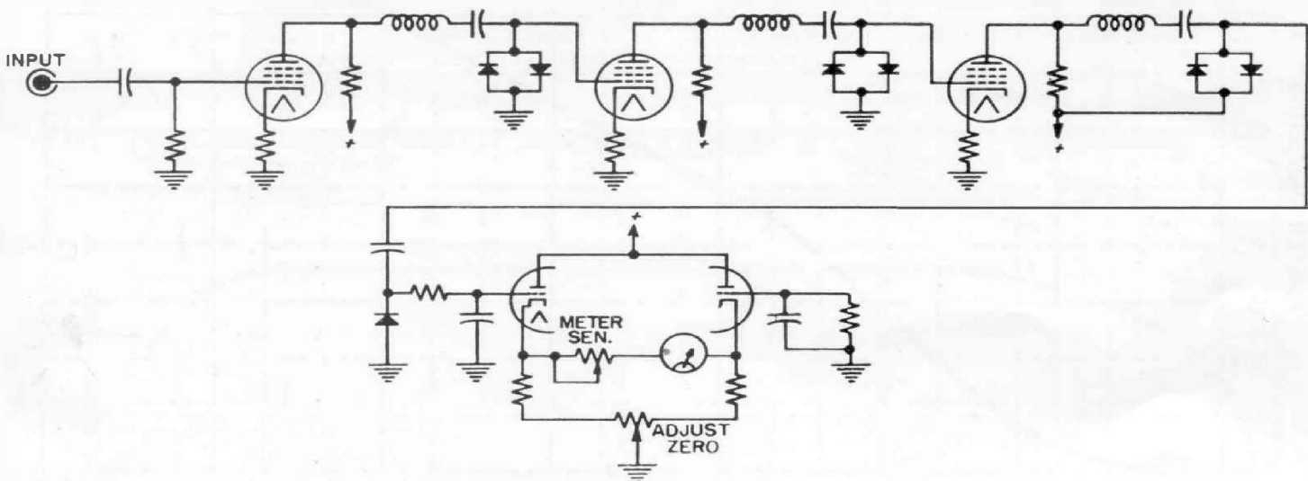
Figure 4. Elementary schematic circuit diagram of the Unit Null Detector.
