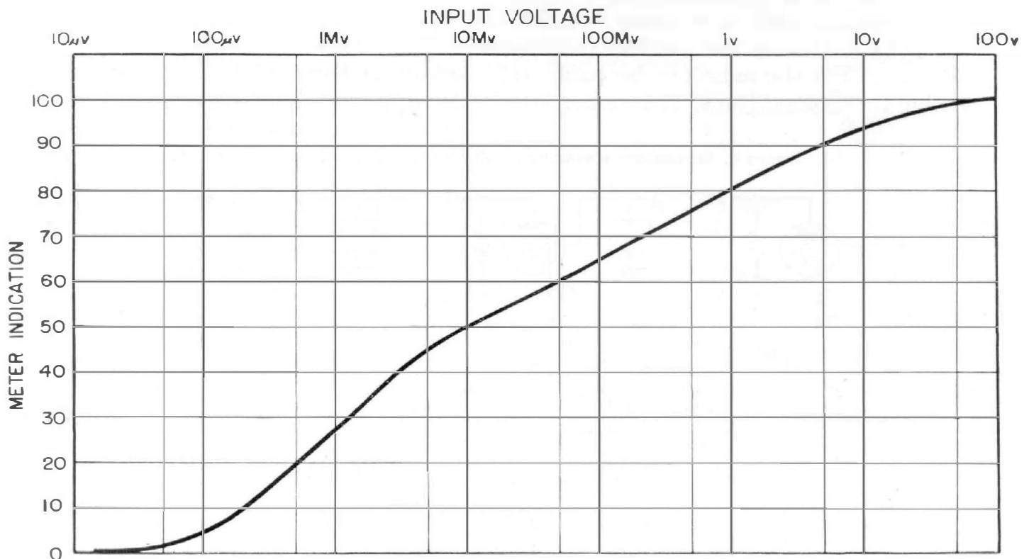
Figure 3. Voltage response curve for the Unit Null Detector.
