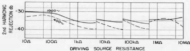
Figure 2. Second harmonic rejection (above) and insertion gain (right) of the Type 1951-A Filter.
